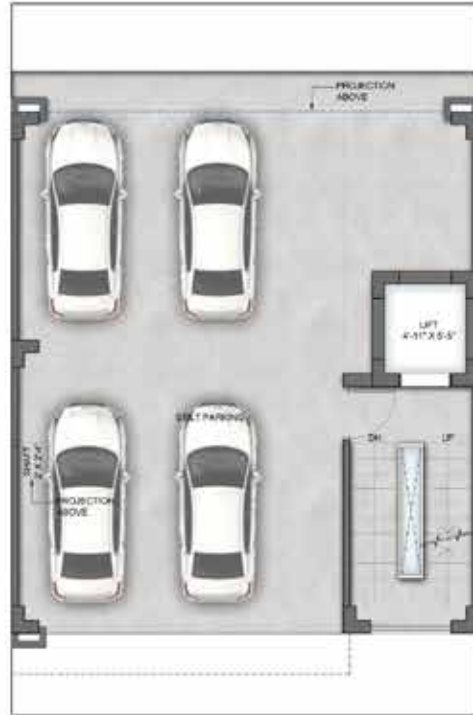
STILT FLOOR PLAN
