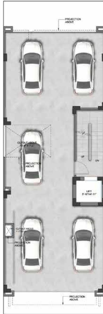
⊖ STILT FLOOR PLAN
